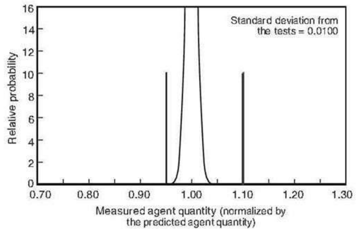
FIGURE A.7.3.3.2(e) Distribution Curve No. 4.
