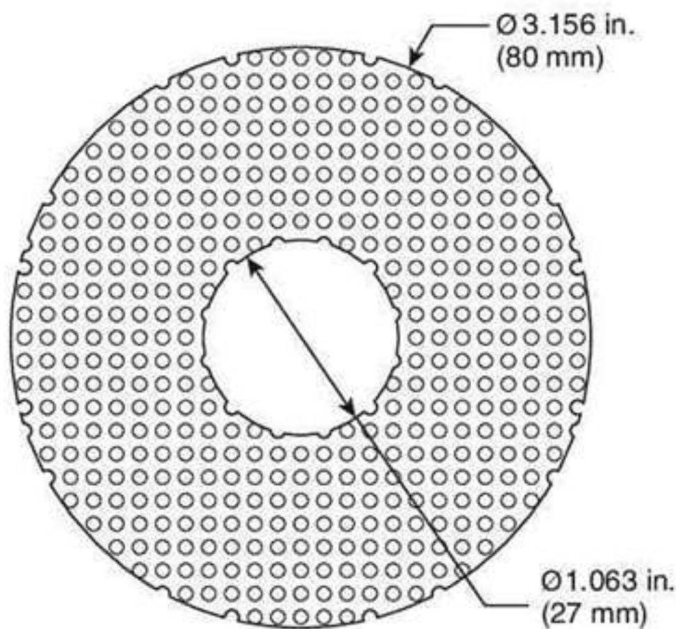
FIGURE C.17(f) Diffuser Bead Support Screen. (Material: 304 SS).
