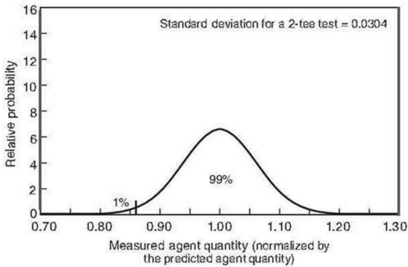
FIGURE A.7.3.3.2(b) Distribution Curve No. 1.
