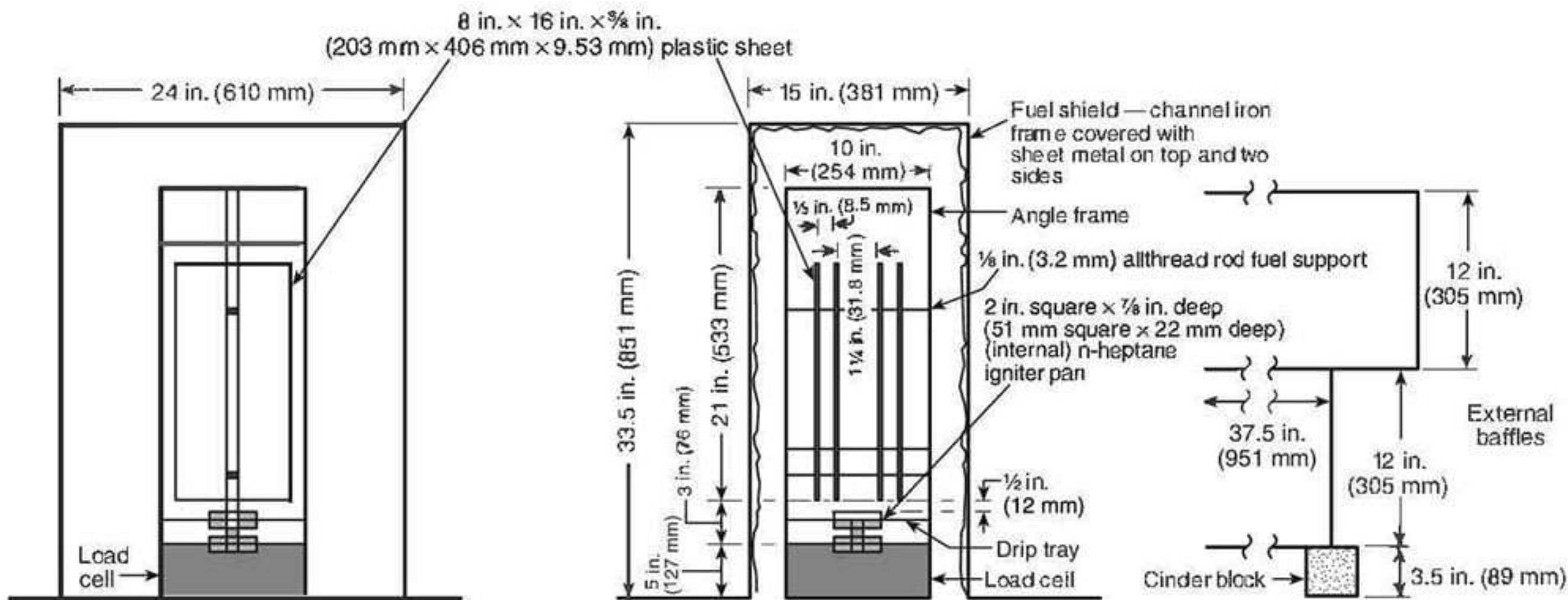
FIGURE A.7.2.2.3(a) Four-Piece Modified Plastic Setup.
