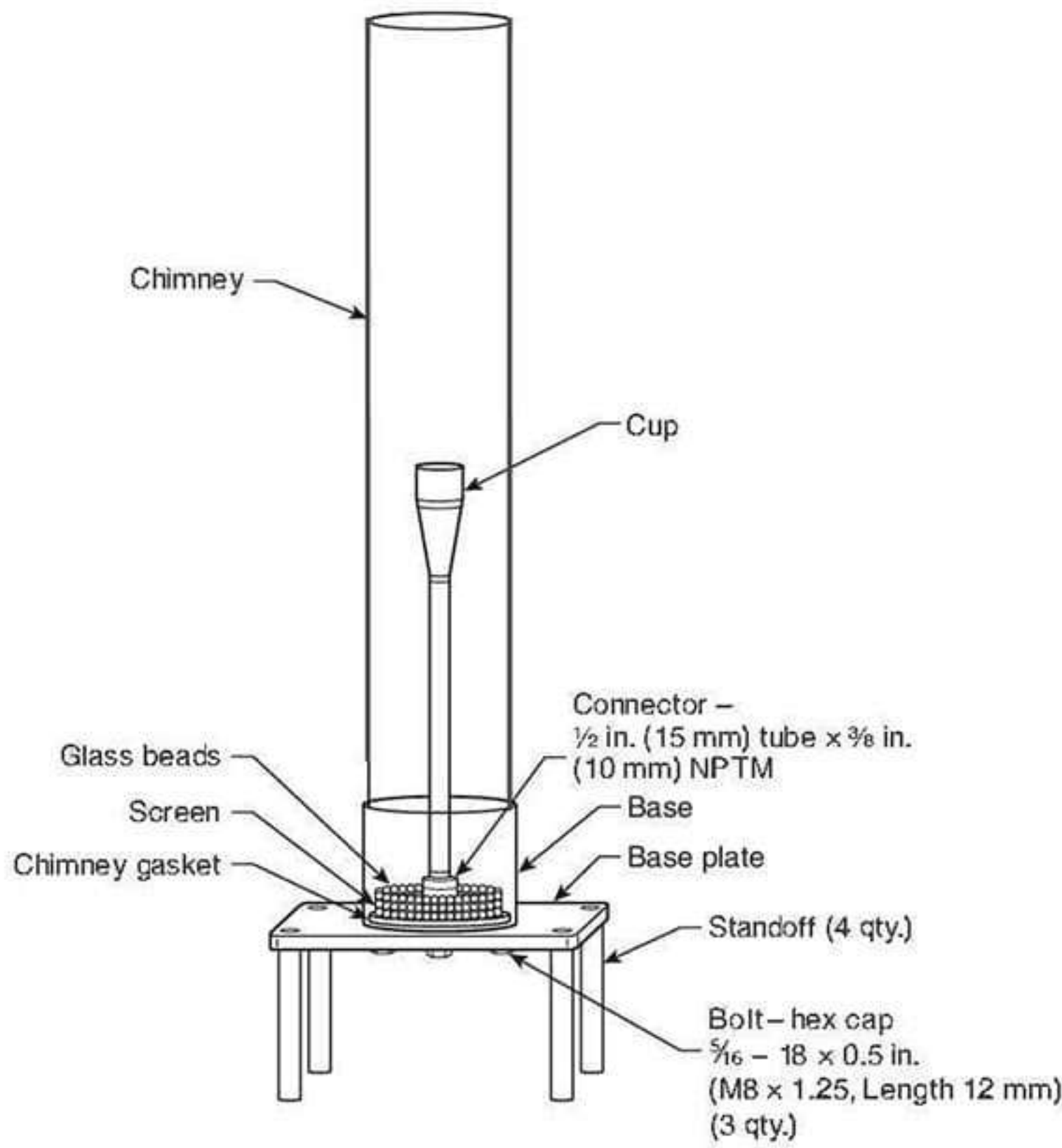
FIGURE C.17(b) Cup Burner Assembly (Transparent View).
