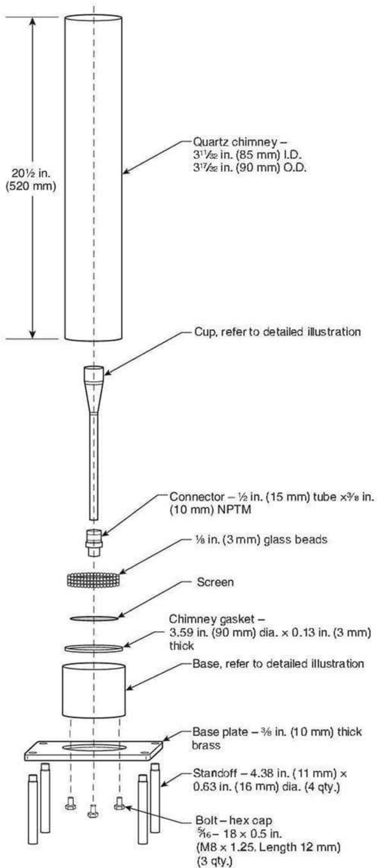
FIGURE C.17(a) Cup Burner Assembly (Exploded View).
