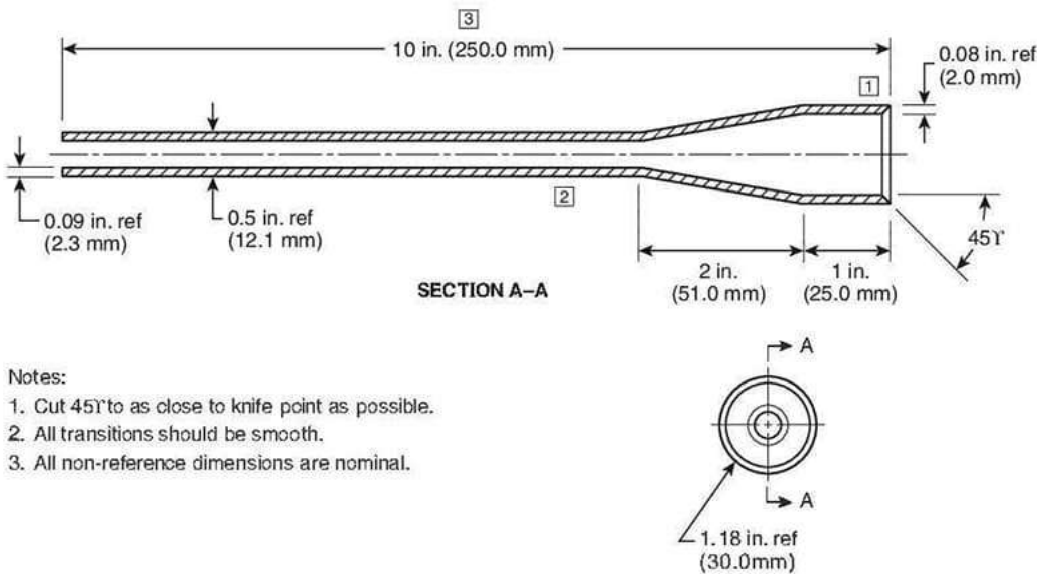
FIGURE C.17(c) Cup Material: Quartz [Dimensions in Inches (Millimeters)].
