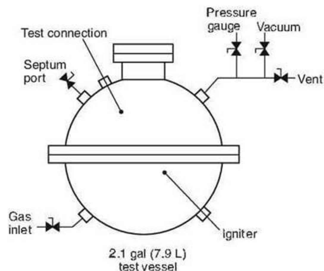
FIGURE A.7.2.3.1 Spherical Test Vessel.
