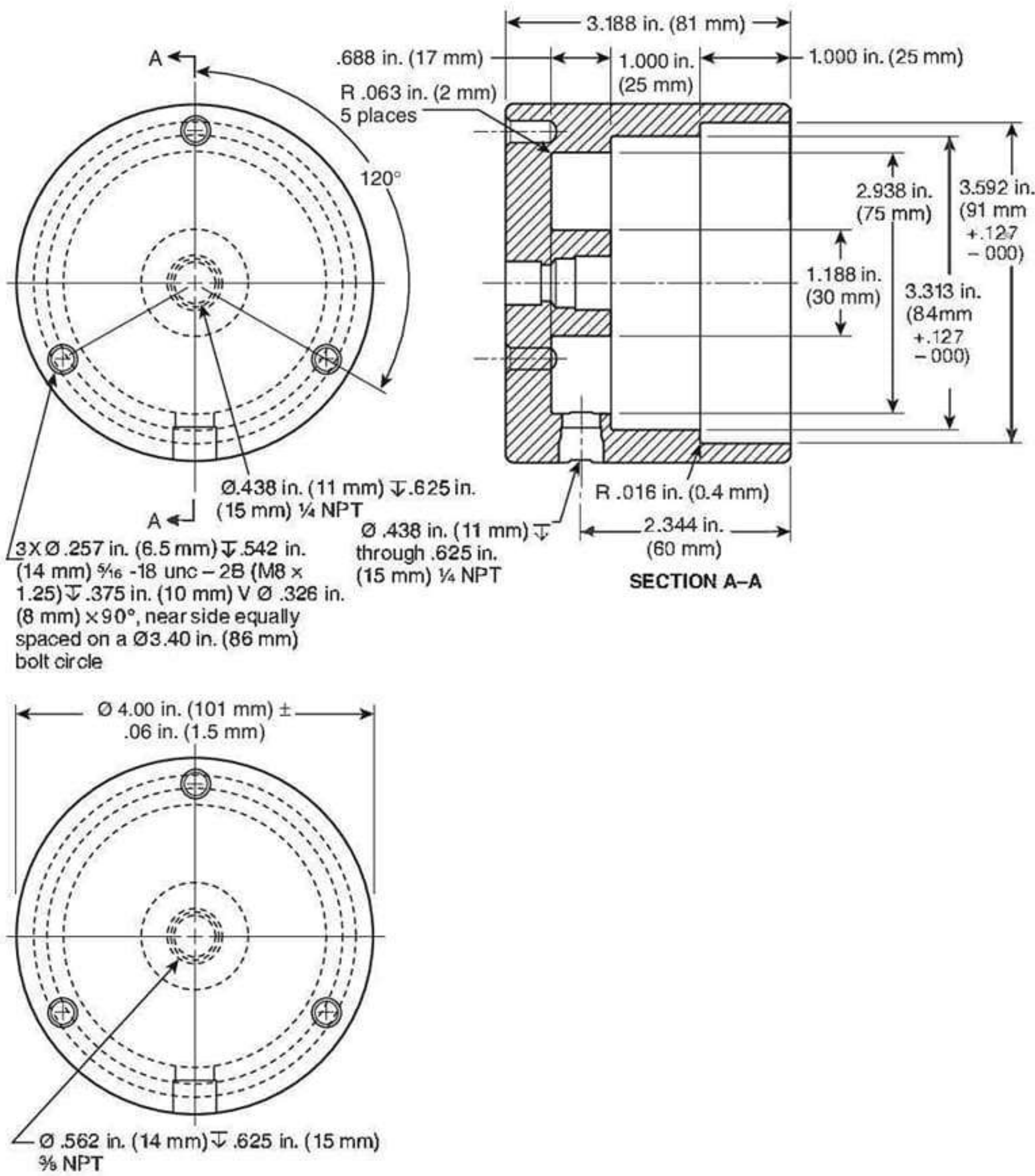
FIGURE C.17(d) Base, Detail.
