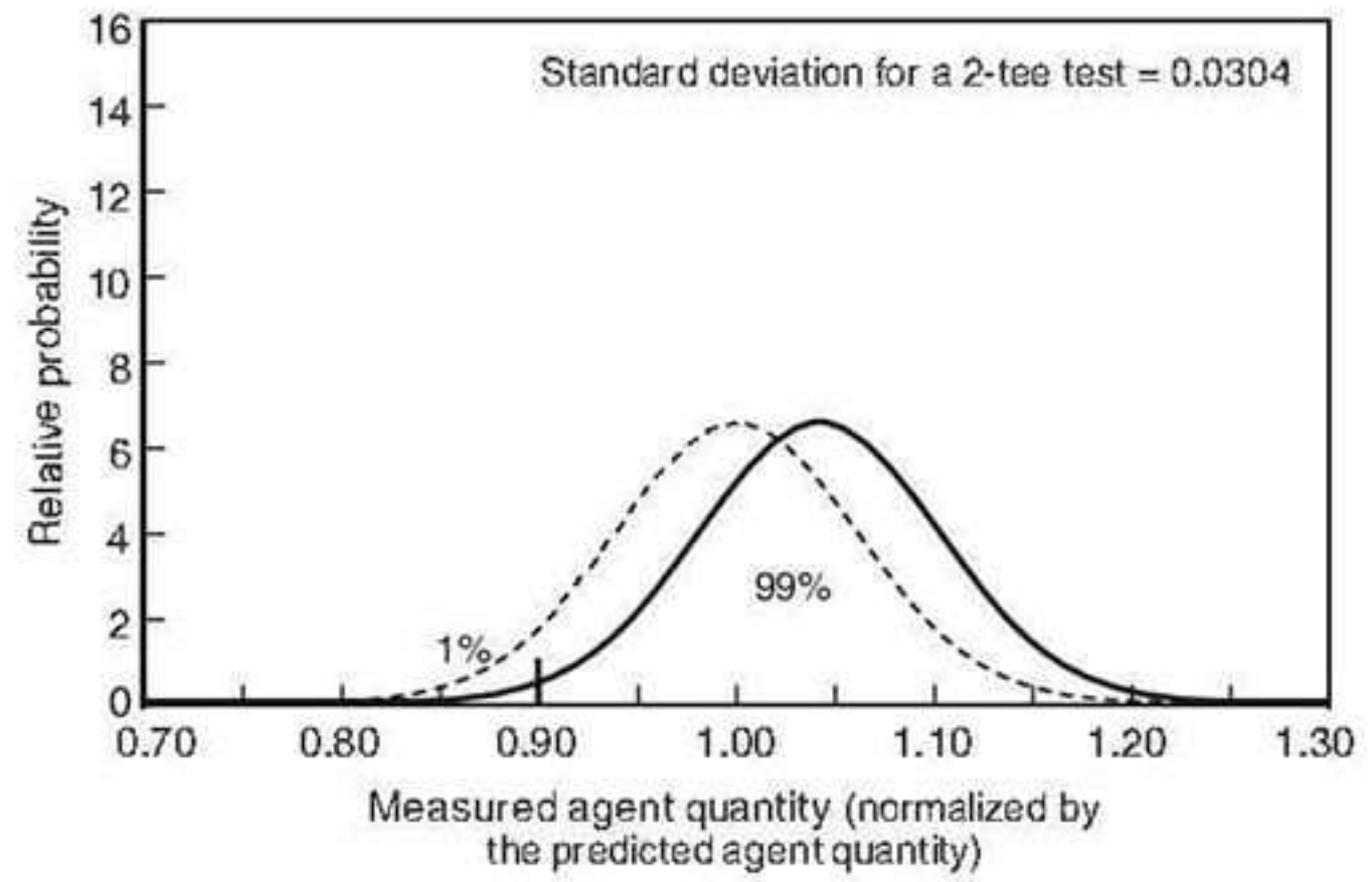
FIGURE A.7.3.3.2(d) Distribution Curve No. 3.
