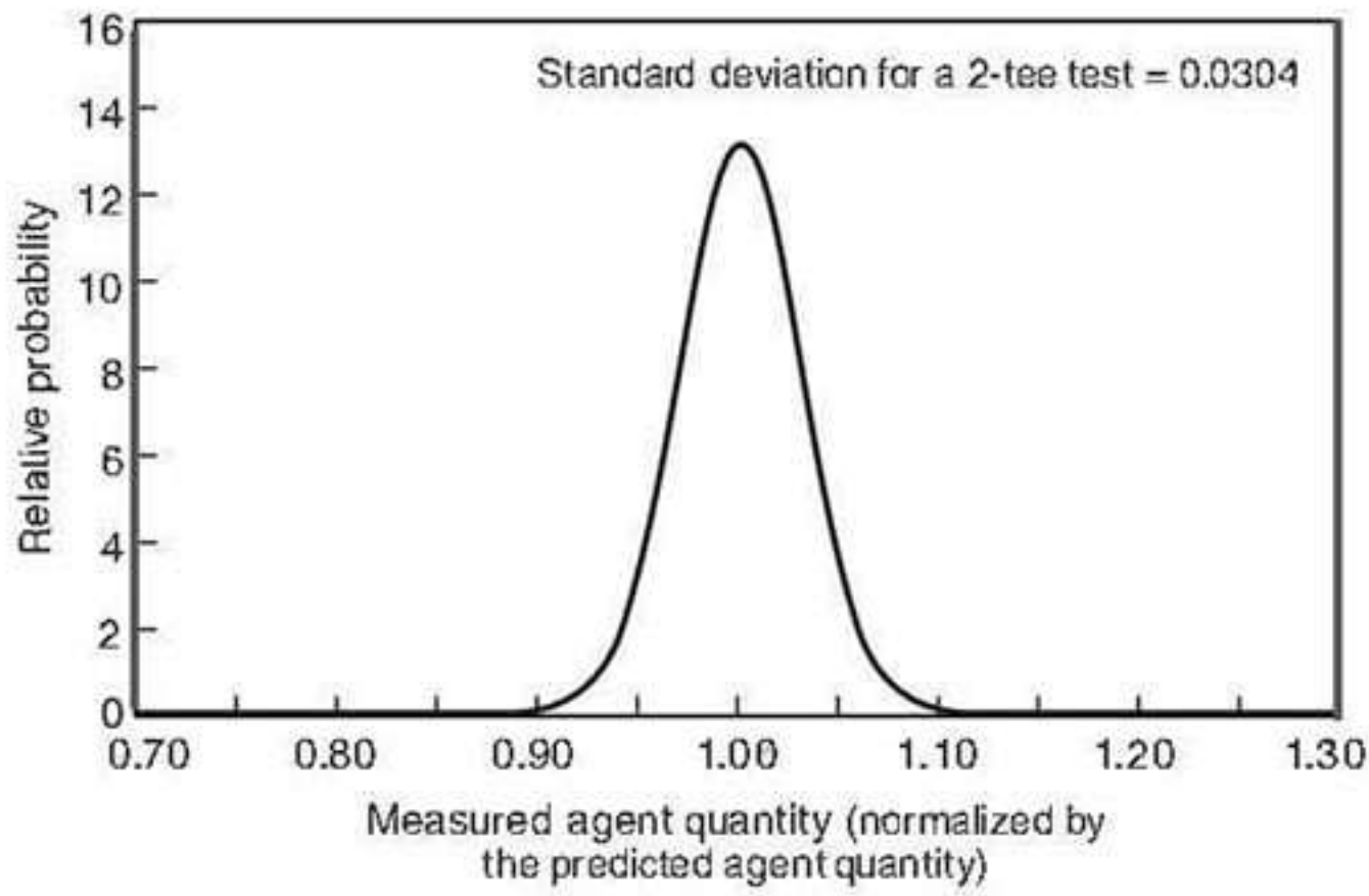
FIGURE A.7.3.3.2(a) Normal Distribution Curve.
