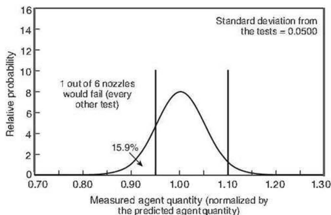
FIGURE A.7.3.3.2(g) Distribution Curve No. 6.
