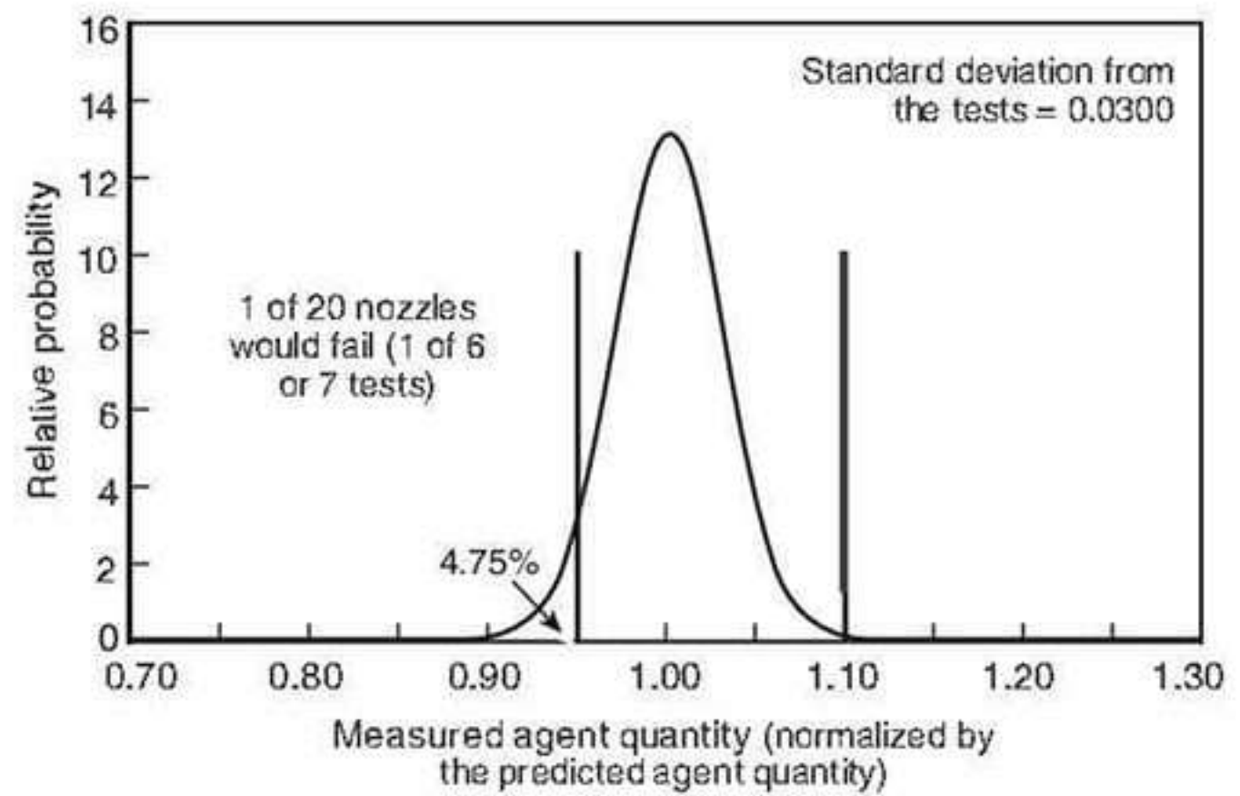
FIGURE A.7.3.3.2(f) Distribution Curve No. 5.
