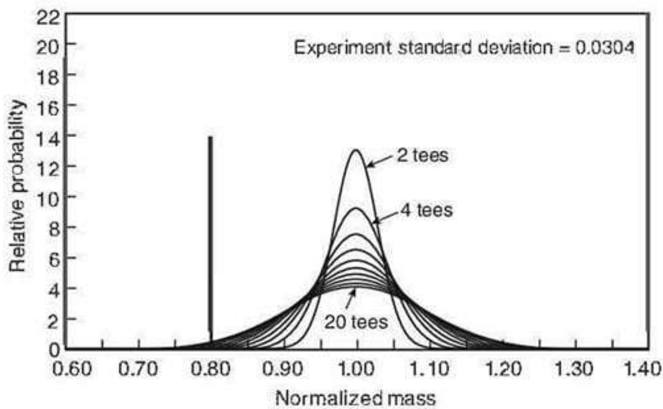
FIGURE A.7.3.3.2(c) Distribution Curve No. 2.
